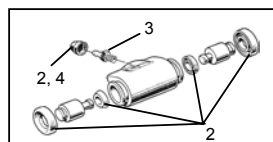
P1800 rear brakes, B18 (Girling)
