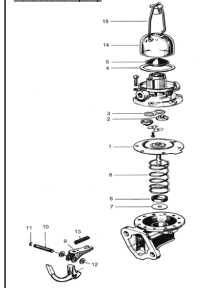
AC Glass-bowl pump
