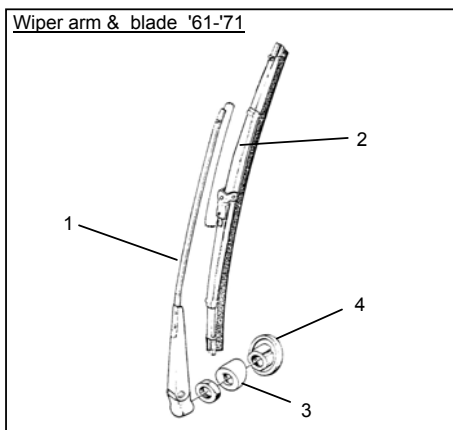
Wiper arm & blade '61-'71
