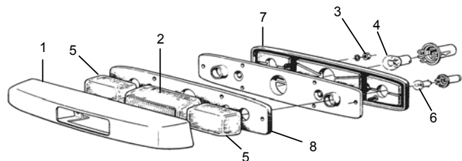
Number-plate lamp assembly, P1800 (from chassis 4200 on)
