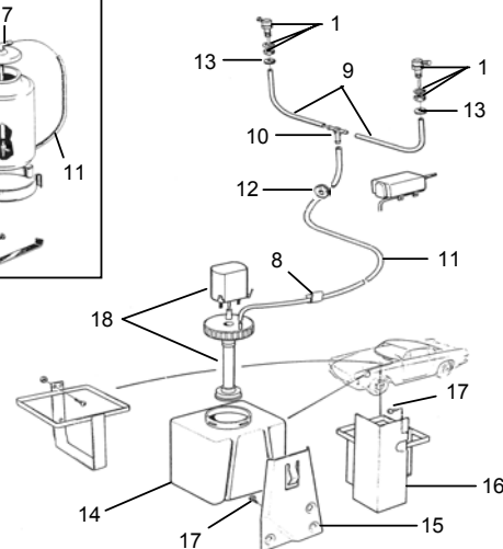
Windscreen Washers, Volvo P1800
