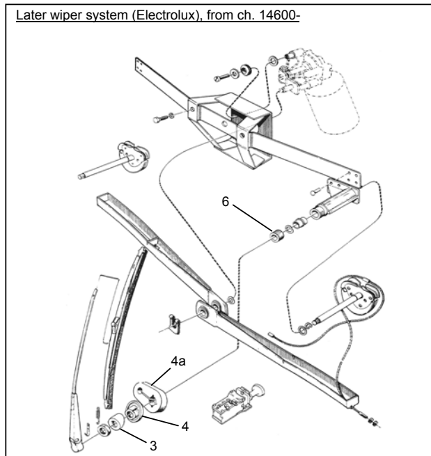
Later wiper system (Electrolux), from ch. 14600-
